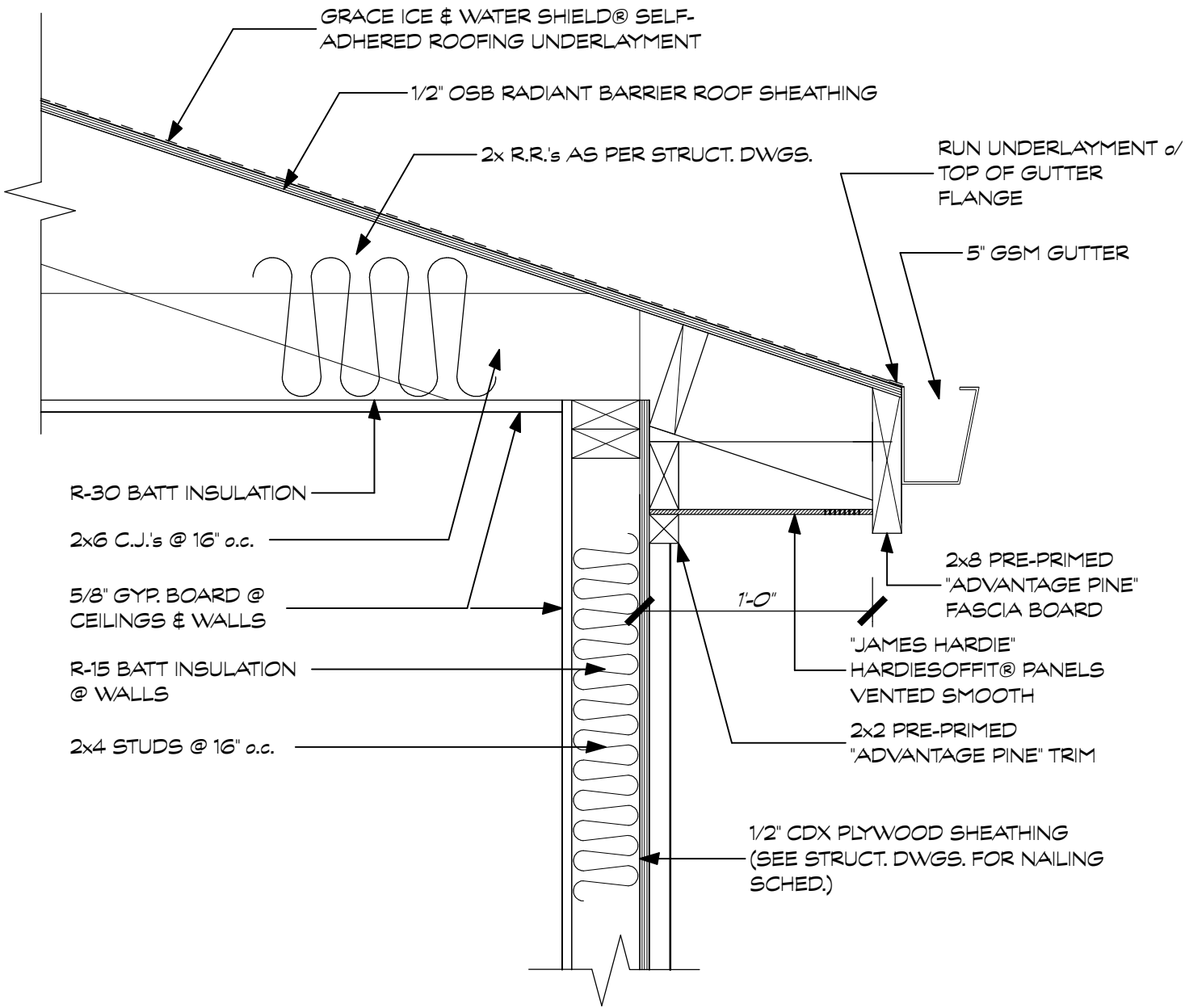
TYPICAL EAVE DETAIL
